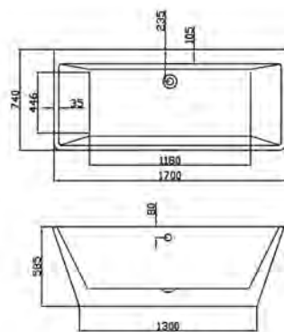
Freestanding-54 1700x740x585mm 67x29.1x23"
