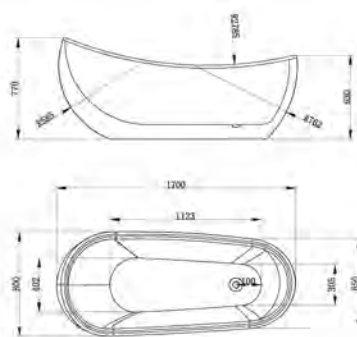
Freestanding-56 1400x800x710mm 55x31x28" 1500x800x740mm 59x31x29" 1600x800x760mm 63x31x30" 1700x800x780mm 67x31x31"
