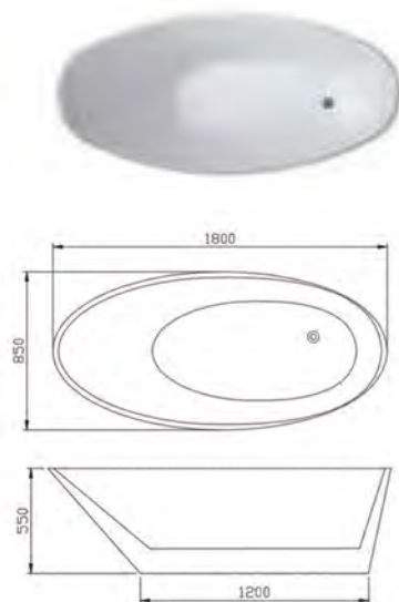
Freestanding-38 1800x850x550mm 70.9x33.5x21.7"
