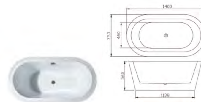
Freestanding-04 1400x750x560mm 55.1x29.5x22" 1500x750x560mm 59x29.5x22" 1600x800x560mm 31.5x29.5x22" 1700x800x600mm 67x27.1x23.6
