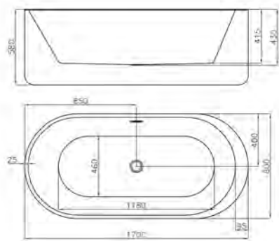
Freestanding-73 1700x800x580mm 67x31x23"
