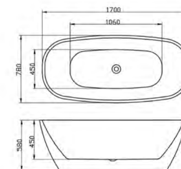
Freestanding-43 1700x780x580mm 67x30.7x22.8"
